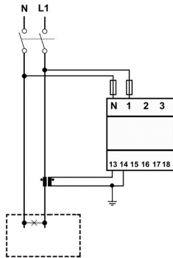
Single-phase installation
