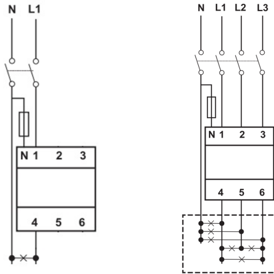
Single-phase installation
