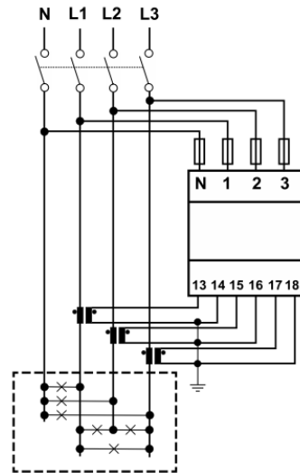
Three-phase installation
